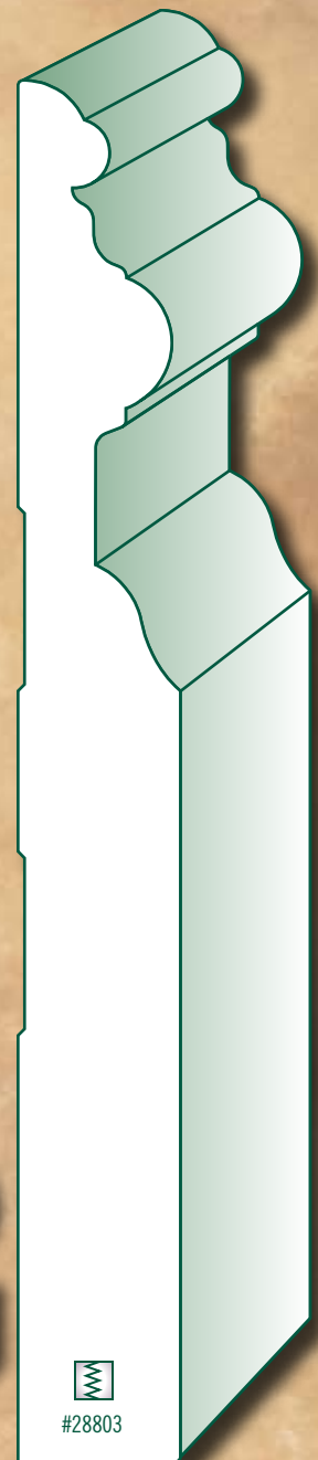
● 6-1/2" Westport Base 3/4 x 6-1/2
