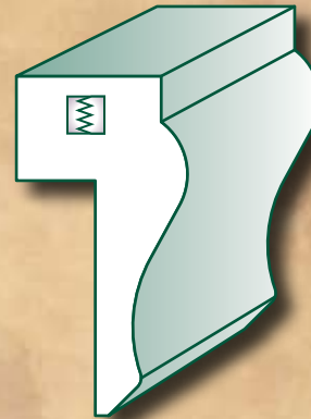
● 1-5/8" Lakeview Chair Rail 13/16 x 1-5/8 #28032
