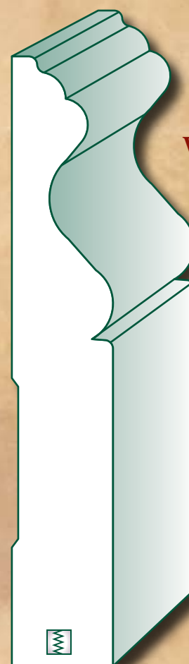
● 4-1/2" Coker Trail Base 3/4 x 4-1/2 #28016
