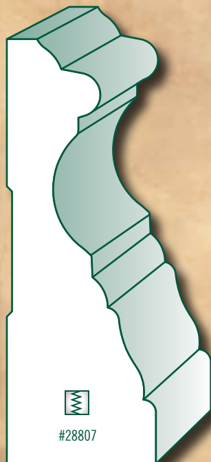
● 3-1/4" Southport Casing 1-1/8 x 3-1/4
