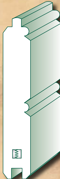
● 1 x 4 T&G Beaded Pine 5/8 x 3-5/16 #28764
