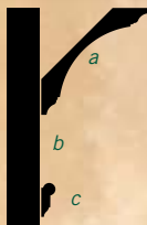
a 7-1/4" Historical Crown 1-3/8 x 7-1/4 b Bare wall painted the same color as the trim c L8288 - Picture Moulding 11/16 x 1-5/8
