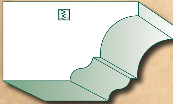
2-1/4" Historical Pediment Crown (HC-1) 2-1/4 x 1-5/16
